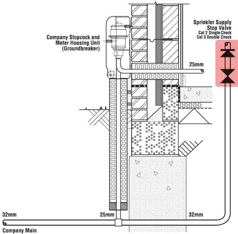
Figure 5 Direct system with groundbreaker wall box
