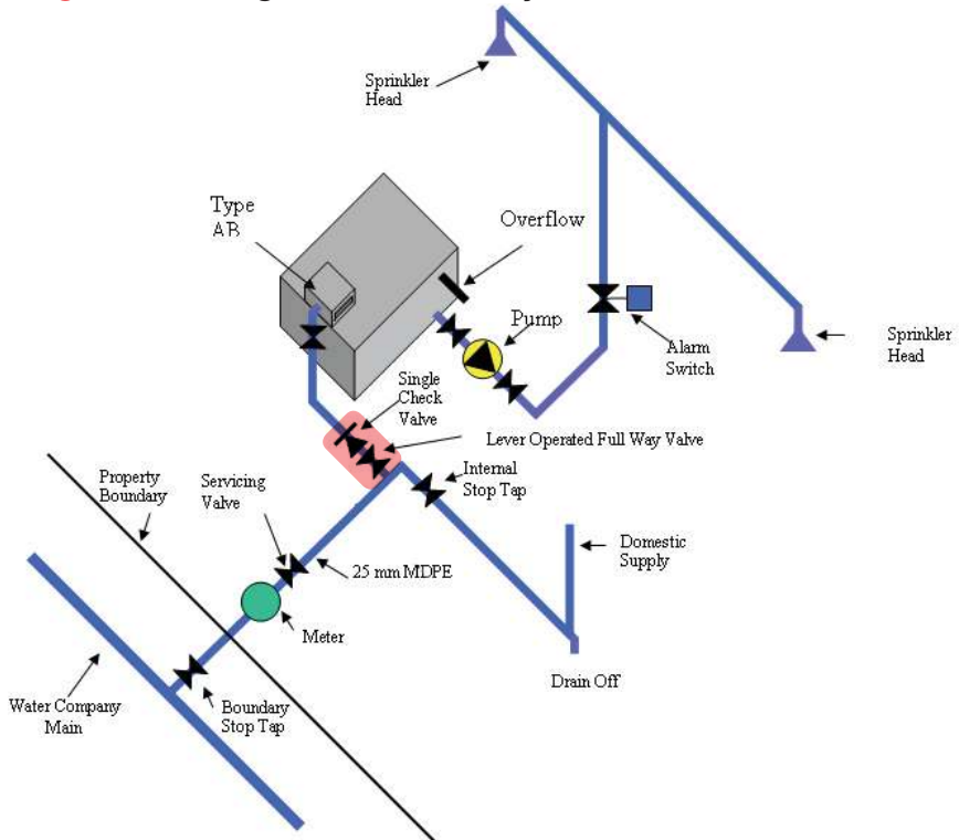
Figure 2 Storage and boosted system
