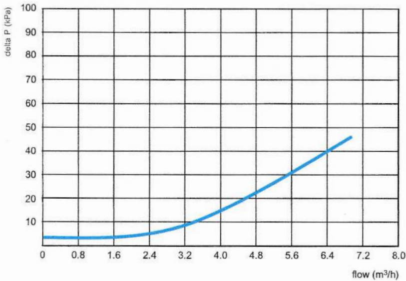
Pressure loss-curve
