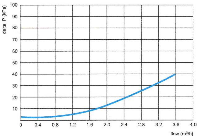
Pressure loss-curve
